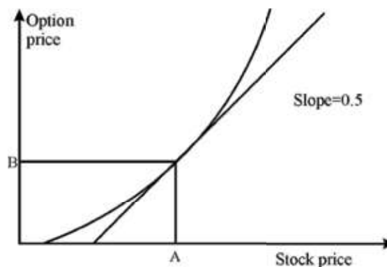
Figure 6.1 \Delta as Slope
